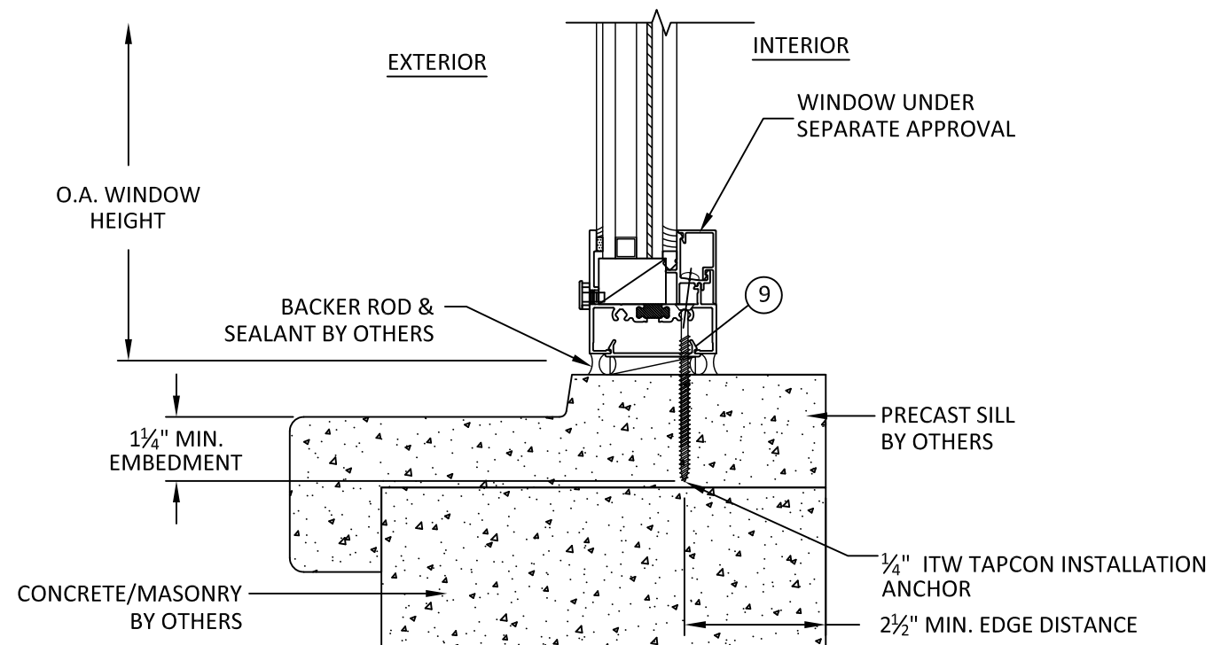
J 3 VERTICAL SECTION SILL - PRECAST SILL UNCLIPPED MULLION
