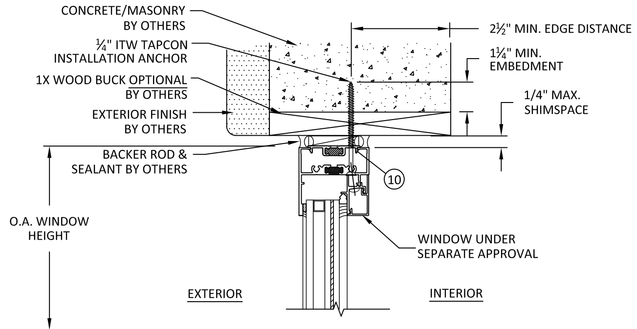
I 3 VERTICAL SECTION HEAD - 1X WOOD BUCK UNCLIPPED MULLION
