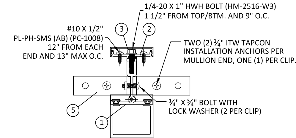
F 2 HORIZONTAL SECTION 2X WOOD MULLION CLIP
