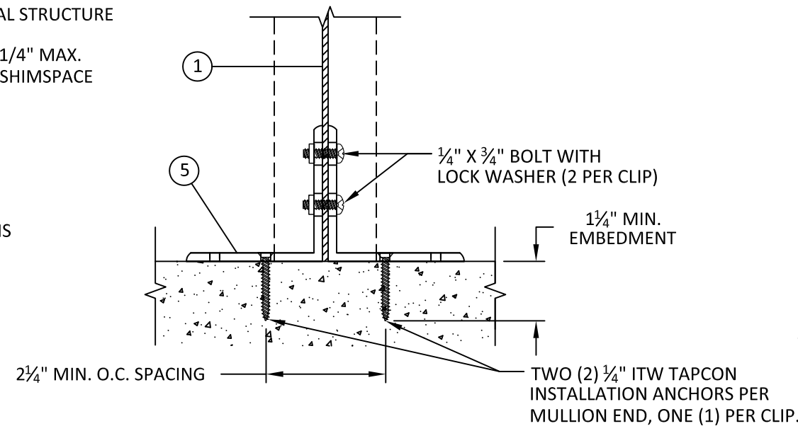
C 2 FRONT VIEW SILL - CONCRETE/MASONRY MULLION CLIP
