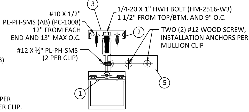
F 2 HORIZONTAL SECTION 2X WOOD MULLION CLIP
