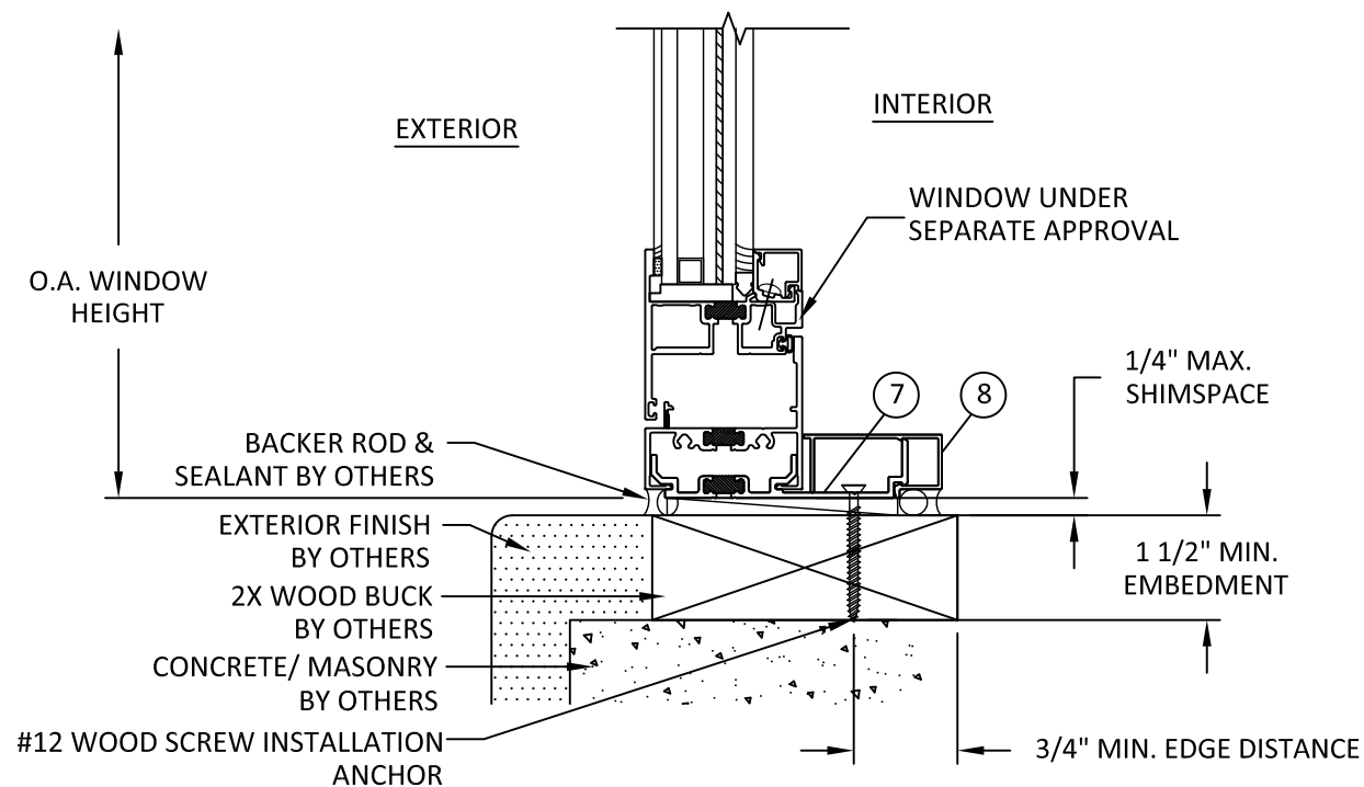
H 3 VERTICAL SECTION SILL - 2X WOOD BUCK UNCLIPPED MULLION (ALT. ANCHOR STRAP)
